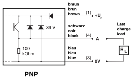
PNP
